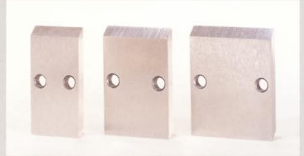
.831" 1.063" 1.281" DOUBLE-HOLE PELLETIZER BLADES
